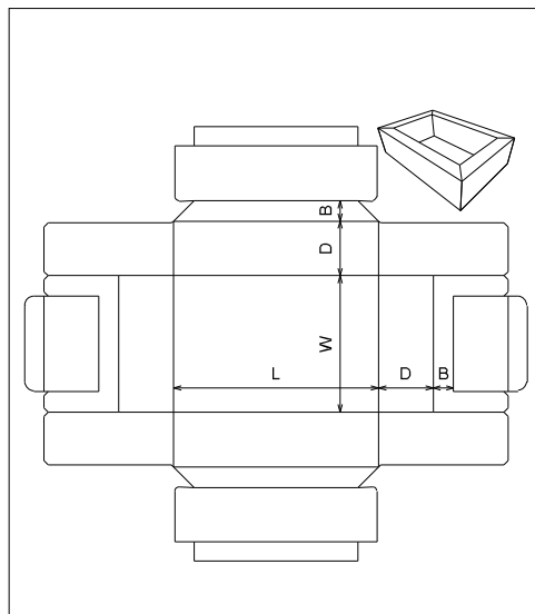
ECMA Folding Carton\Group B\ECMA B1410 - FC0305 - Buffer Wall Tray
