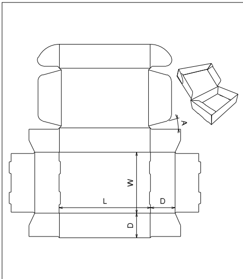
ECMA Folding Carton\Group B\ECMA B2150 Style B - FC0312 - Turn Over Hinged Lid B
