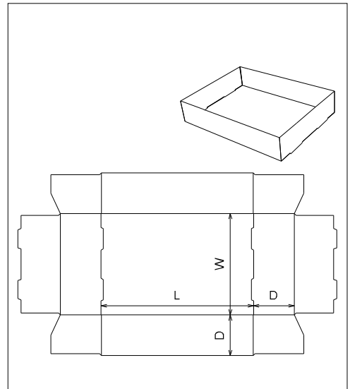
ECMA Folding Carton\Group B\ECMA B2110 - FC0304 - Turn Over End Tray
