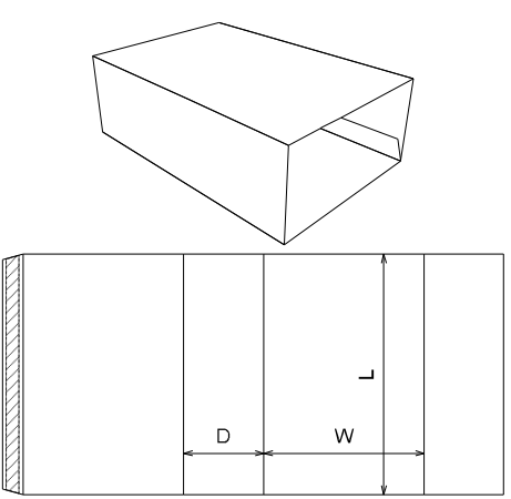
ECMA Folding Carton\Group E\ECMA E3120 Style C - FC0403 - Sleeve With/Without Thumb Cuts
