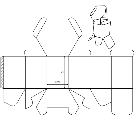
ECMA Folding Carton\Group C\ECMA C4055 - FC0606 - Hexagonal Snap Lock Base
