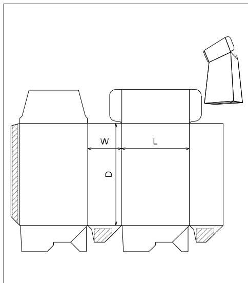
ECMA Folding Carton\Group A\ECMA A6040 - FC0116 - Side Tuck Crash Lock Base
