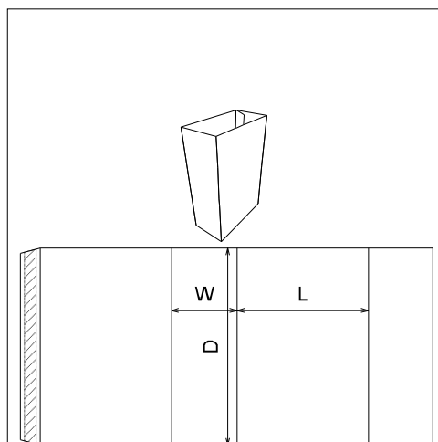
ECMA Folding Carton\Group A\ECMA A1010 - FC0504 - Square Flap Skillet
