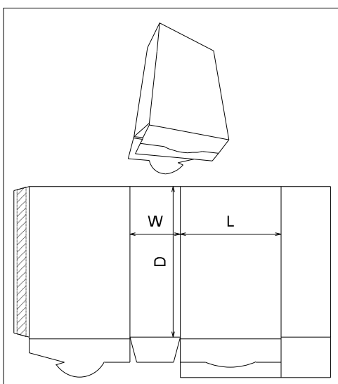
ECMA Folding Carton\Group A\ECMA A5601 Style A - Open Ended Locking Skilllet
