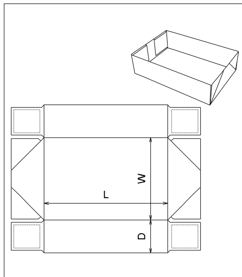
ECMA Folding Carton\Group B\ECMA B4020 Style A - FC0301 In-Fold Tray, 4 Corner Glued
