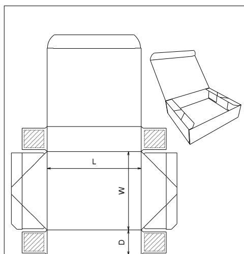
ECMA Folding Carton\Group B\ECMA B4050 - FC0308 - Four Corner Hinged Lid
