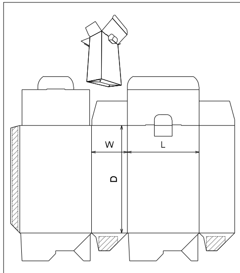
ECMA Folding Carton\Group A\ECMA A6098 - FC0110 - Double Tuck Crash Lock Base
