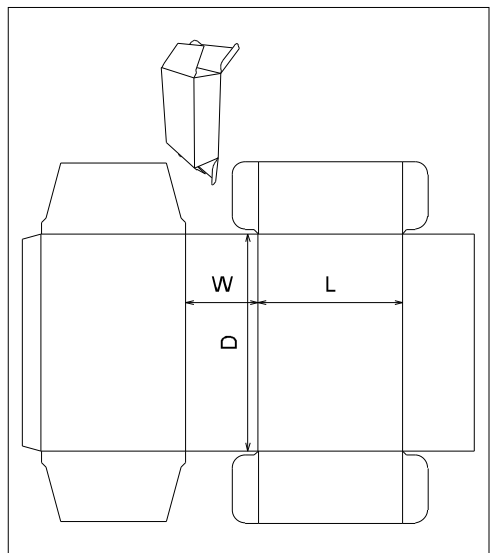
ECMA Folding Carton\Group A\ECMA A4040 - FC0208 - Side Tuck Top and Base
