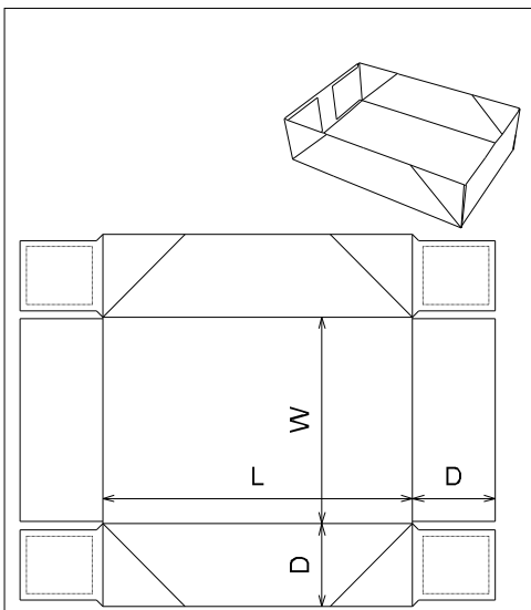
ECMA Folding Carton\Group B\ECMA B4020 Style B - FC0302 - Out-Fold Tray
