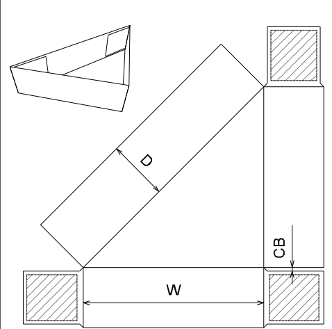
ECMA Folding Carton\Group D\ECMA D1010 - Triangular Single-Walled Carton
