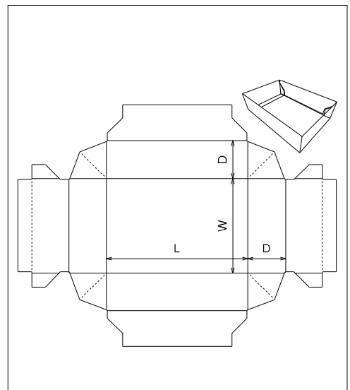
ECMA Folding Carton\Group B\ECMA B1021 - FC0307 - Shirt Box Style
