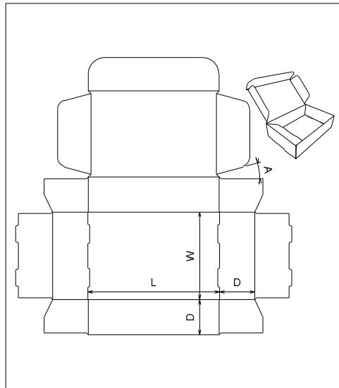
ECMA Folding Carton\Group B\ECMA B2150 Style A - FC0311 - Turn Over Hinged Lid A
