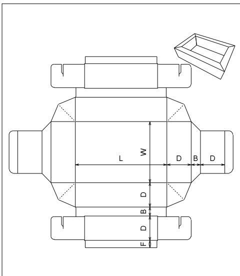
ECMA Folding Carton\Group B\ECMA B1411 - FC0306 - Buffer Wall Tray with Webbed Corners
