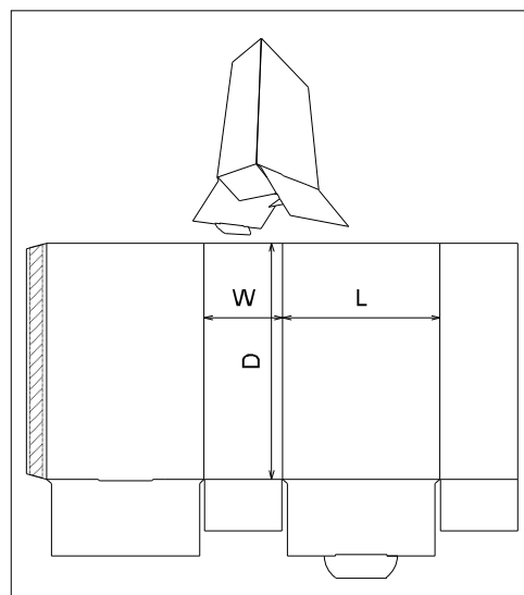
ECMA Folding Carton\Group A\ECMA A5601 Style B - Open Top Edge Lock Skilllet
