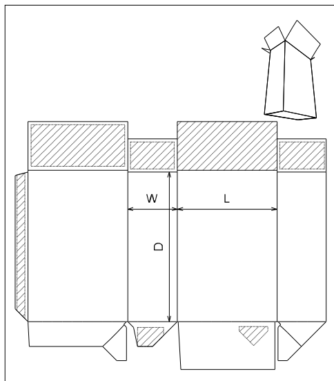
ECMA Folding Carton\Group A\ECMA A6110 - FC0123 - Square Skillet Full Crash Lock Base
