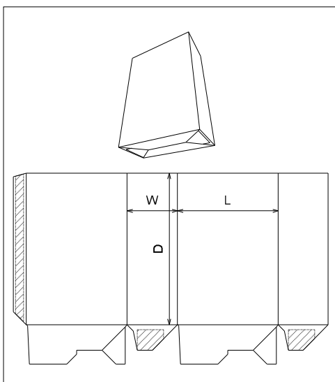
ECMA Folding Carton\Group A\ECMA A6001 - FC0125 - Open Ended Crash Lock Base
