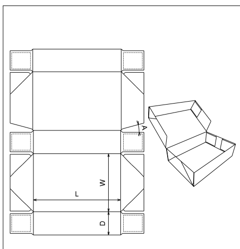
ECMA Folding Carton\Group B\ECMA B6020 - FC0310 6 Corner Glued Tray with Hinged Lid
