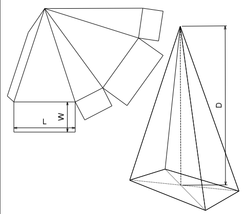
ECMA Folding Carton\Group C\ECMA C2210 - Rectangular Base Pyramid with Square Flaps
