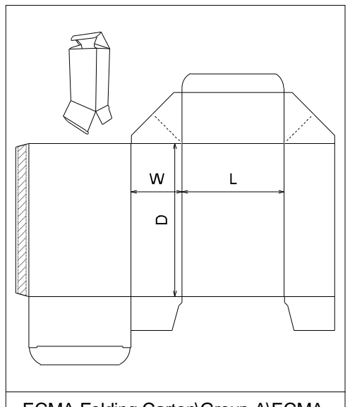
ECMA Folding Carton\Group A\ECMA A2299 - FC0223 - Webbed Tuck Tuck to Front
