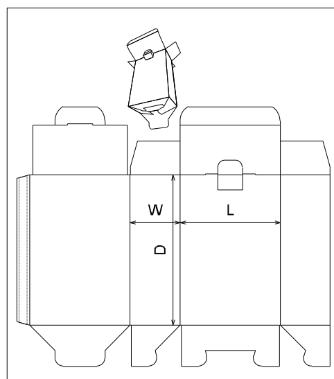
ECMA Folding Carton\Group A\ECMA A5598 - FC0112 - Double Tuck Snap Lock Base
