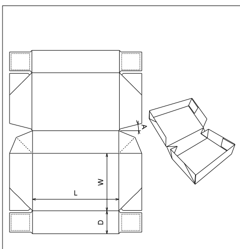
ECMA Folding Carton\Group B\ECMA B6121 - FC0309 Four Corner Hinged Lid with Webbed Corners
